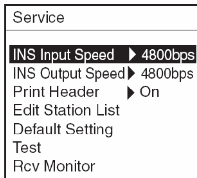
Меню Service
